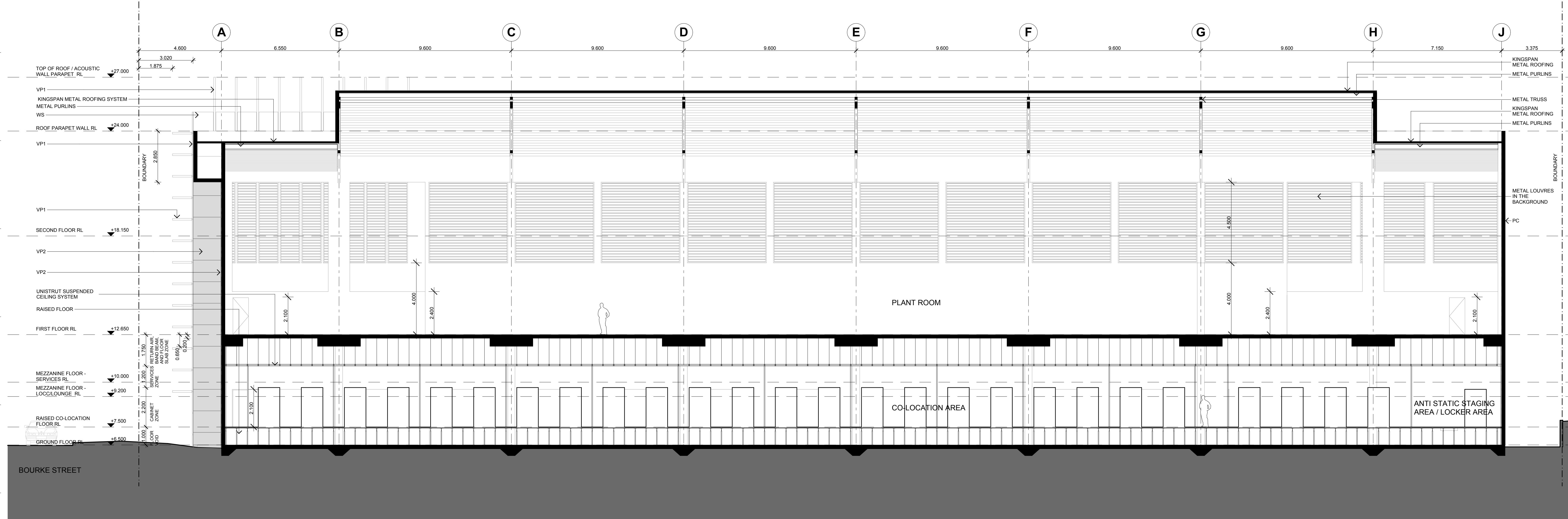
SECTION B
